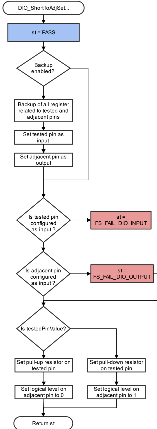
Figure 23. Block diagram of FS_DIO_ShortToAdjSet_RGPIO() function IEC60730_B_CM4_CM7_Library_UG_v4_3, Rev. 0, 30 September 2022
