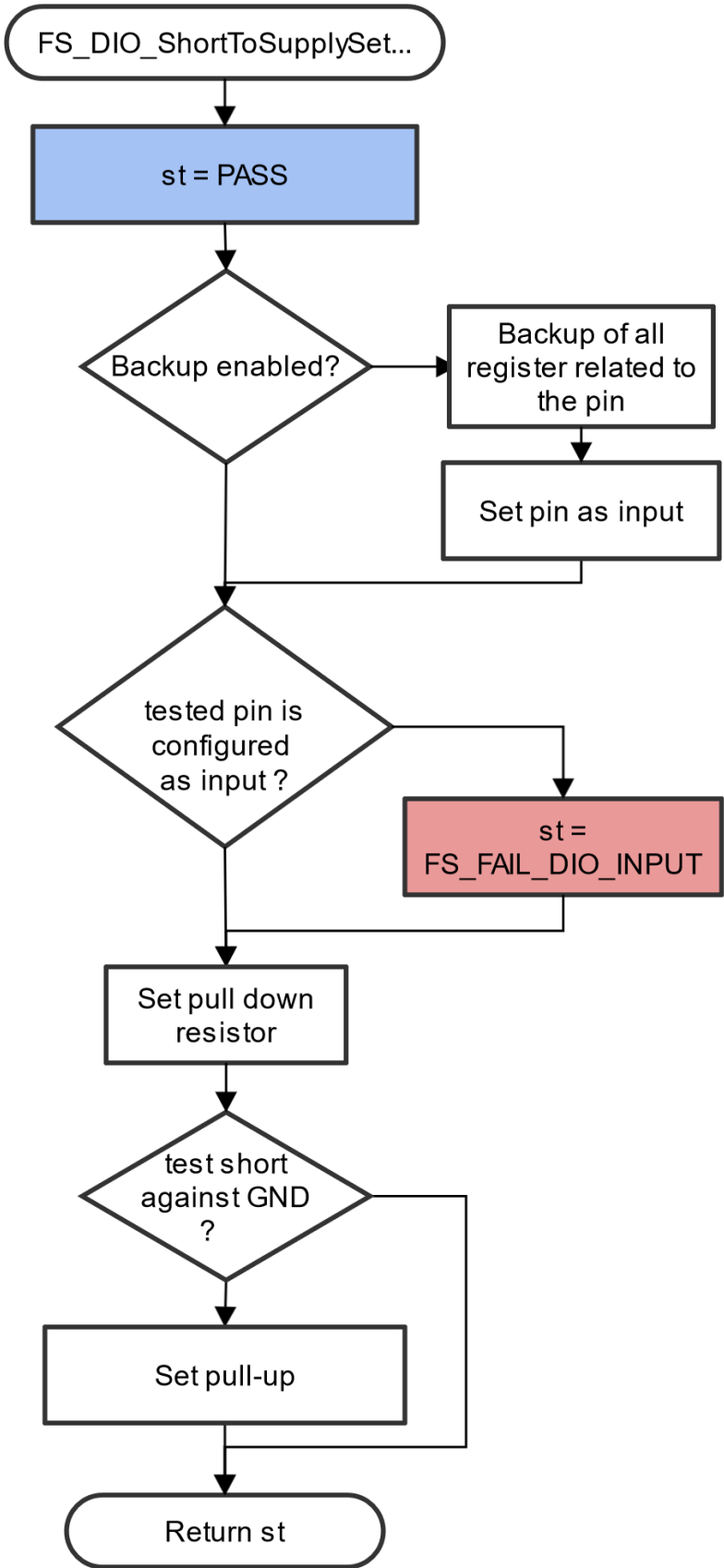
Figure 13. Block diagram of FS_DIO_ShortToSupplySet_IMX8M0 function IEC60730_B_CM4_CM7_Library_UG_v4_3, Rev. 0, 30 September 2022
