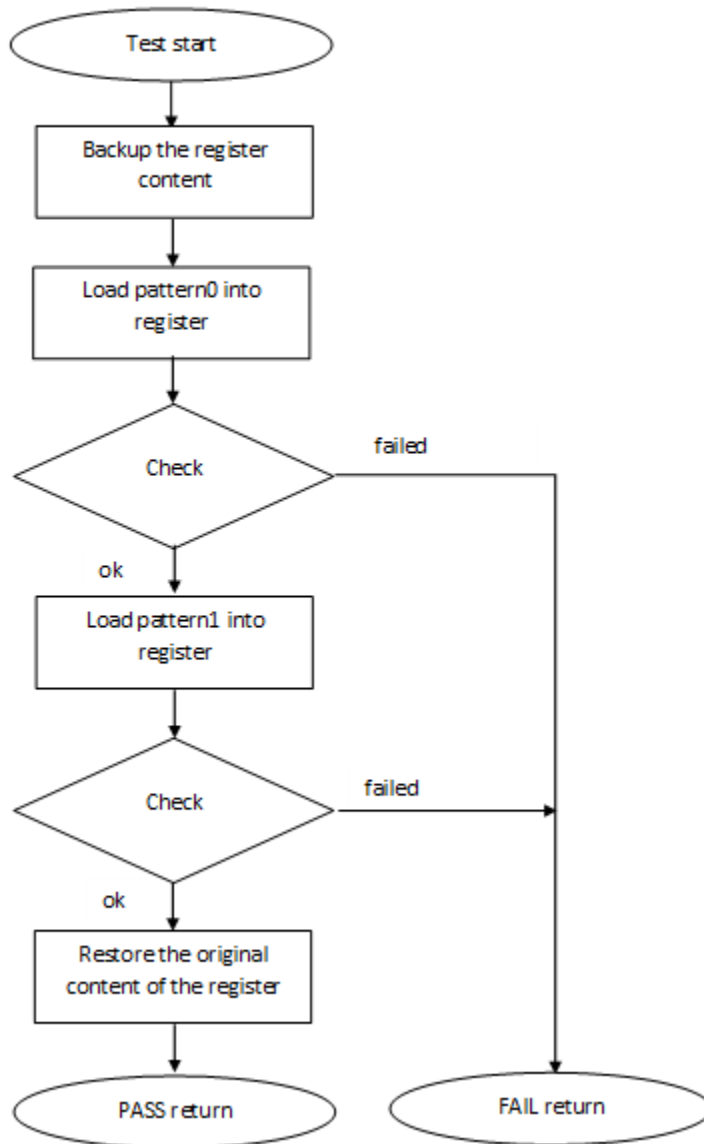
Figure 31. Block diagram for PRIMASK , FAULTMASK, BASEPRI and CONTROL registers test
