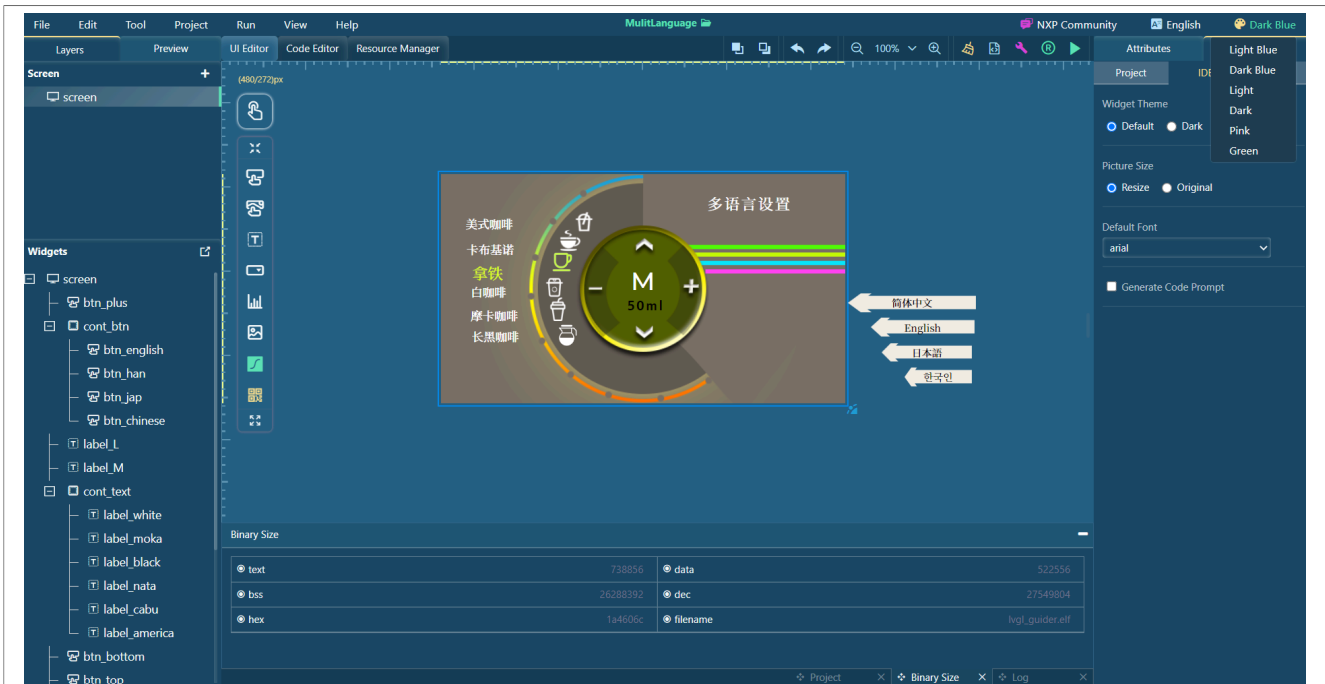
Figure 27. IDE setting
