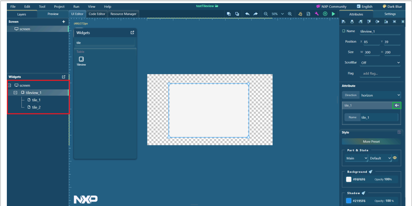
Figure 110. Button widget
