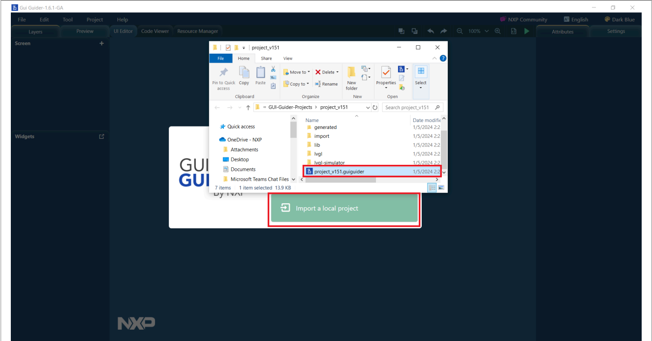
Figure 116. Open project
